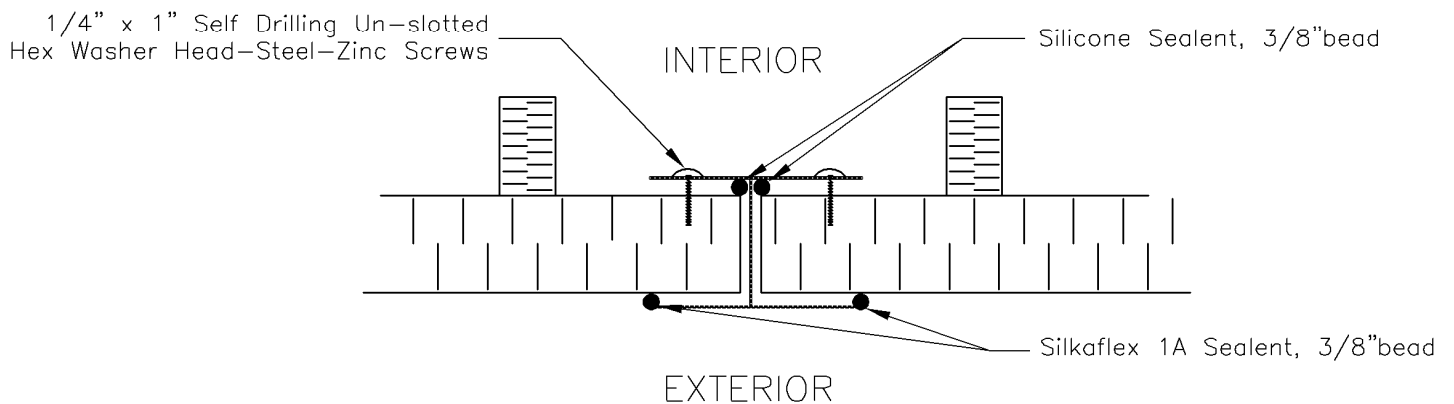
Figure 2: Below Grade Use Joint Protection Details
